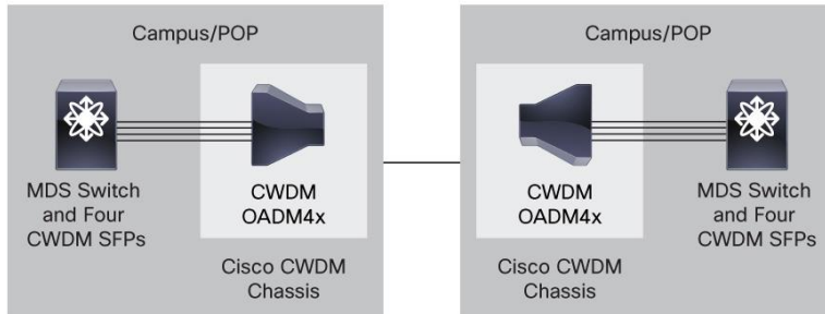
Figure 13. Point-to-Point Architecture (Dual-Fiber Link)
