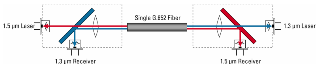
Figure 3. Bidirectional Transmission of a Single Strand of SMF
