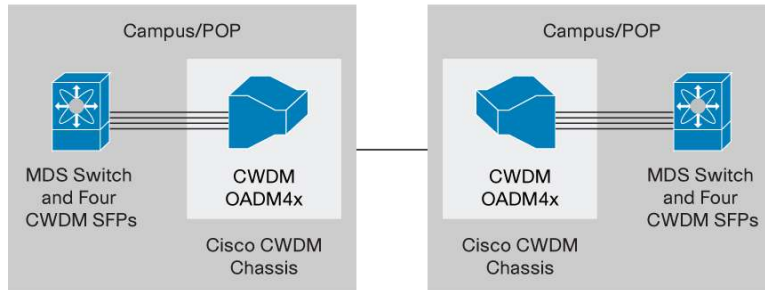
Figure 12. Point-to-Point Architecture (Dual-Fiber Link)
